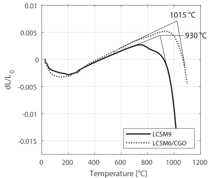
Figure S1: Dilatometry measurements showing the shrinkage of slip-cast LCSM9 and LCSM6/CGO pellets during densification. Onset temperatures have been evaluated by analyzing shrinkage curves using Proteus Thermal Analysis software (NETZSCH) and are indicated in the plot.
